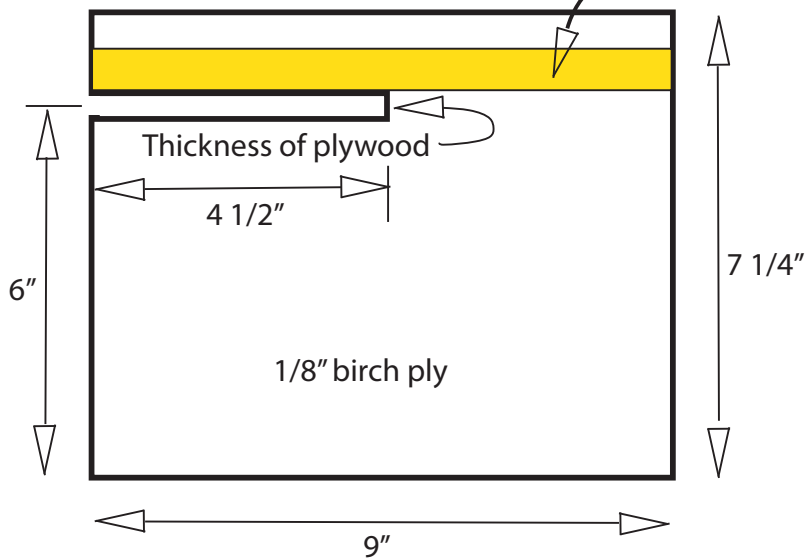
non-slip shelf liner material 1"x9" glued on with rubber cement
